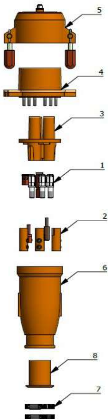
MALE COUPLER
