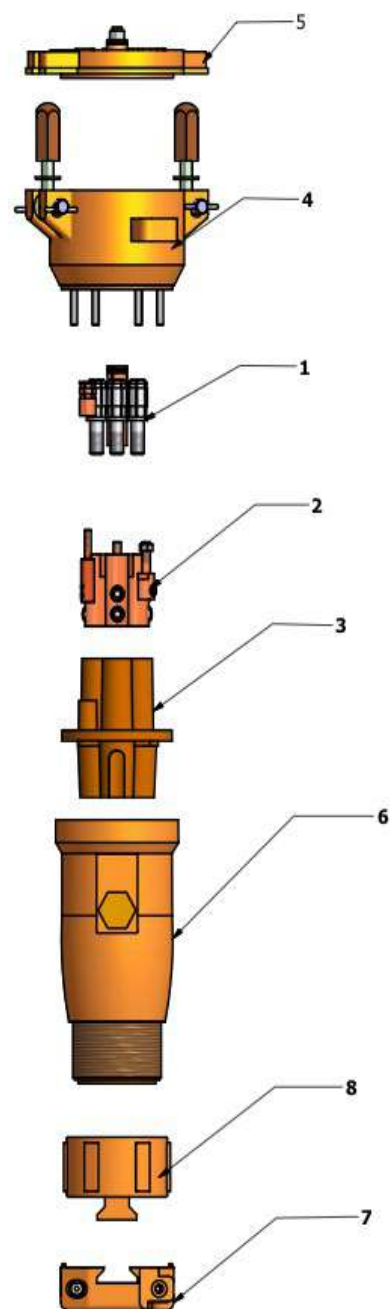
FEMALE COUPLER
