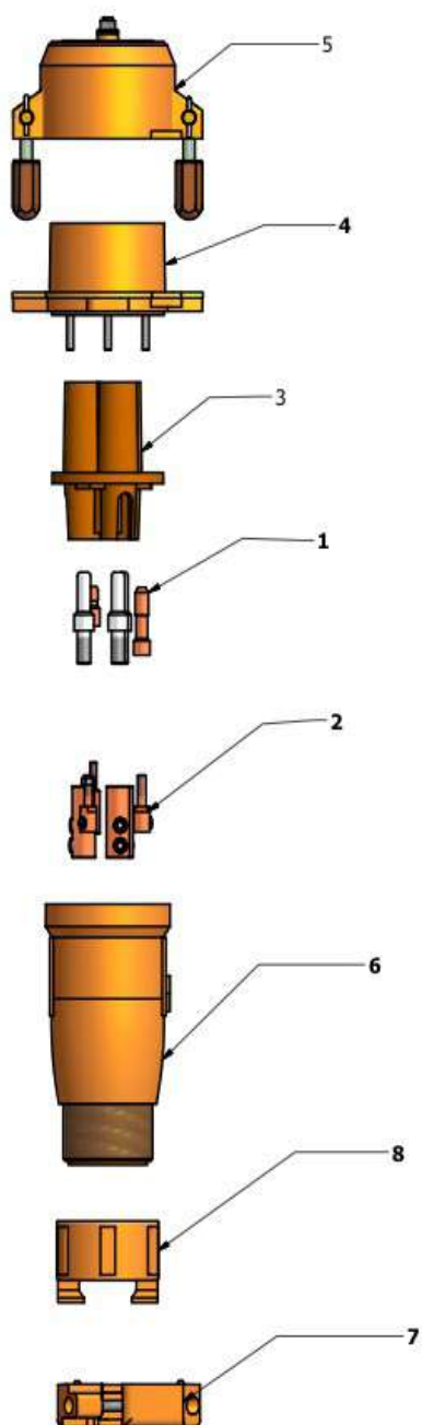
MALE COUPLER
